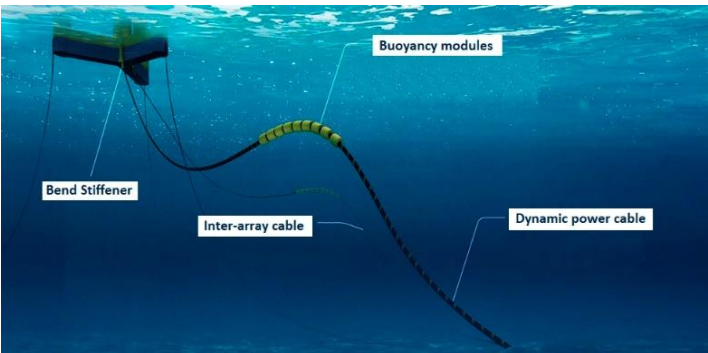
Figure 6: Illustration of the inter-array cable or dynamic power cable and its buoyancy modules and bend stiffener (stiffener located at the connection to the floating system) © RTE
