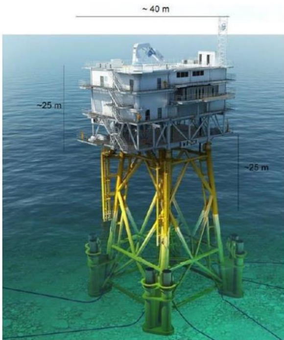
Figure 8: Illustration of the offshore electrical substation of Westermost Rough (England) © Chantier de l'Atlantique
