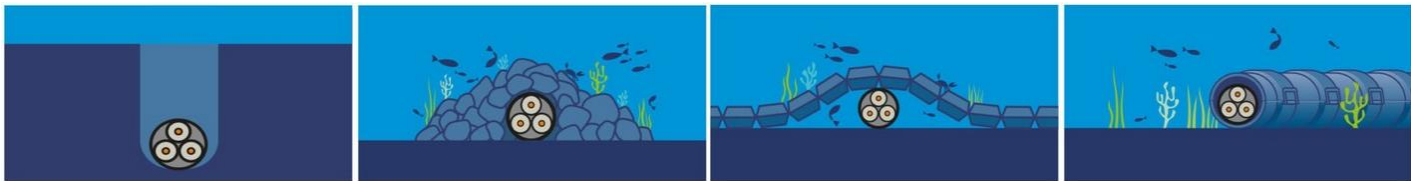
Figure 7: Illustration of the different type of cable protection. From left to right: Buried, Riprap, Concrete mats, and Protective shells © RTE
