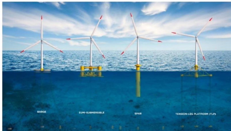
Figure 3: Illustration of the different categories of floating infrastructures © WindEurope
